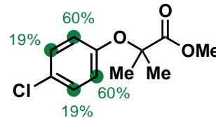
5. Clofibrate
