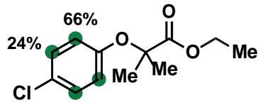
12. Clofibrate
