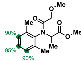
9. Metalaxyl
