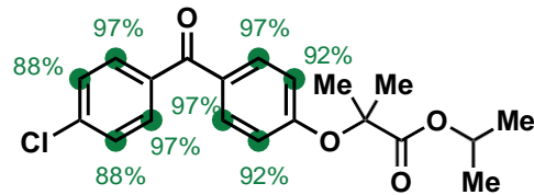
4. Fenofibrate
